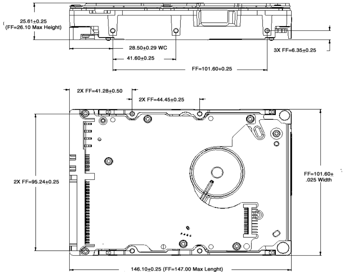
Figure 3-6 Mounting Dimensions Maxtor Atlas 15K II Drives
