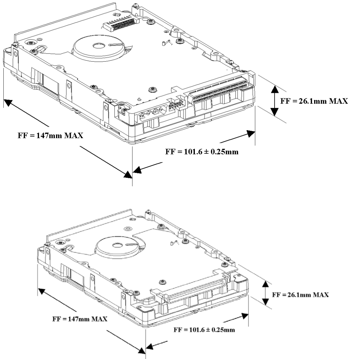
Figure 3-1 Dimensions for the Maxtor Atlas 15K II Hard Disk Drives
