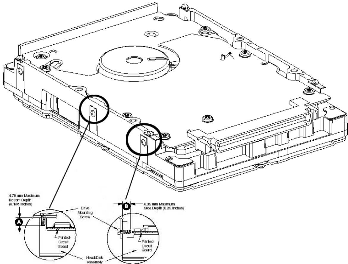
Figure 3-7 Mounting Screw Clearance for Maxtor Atlas 15K II Drive
