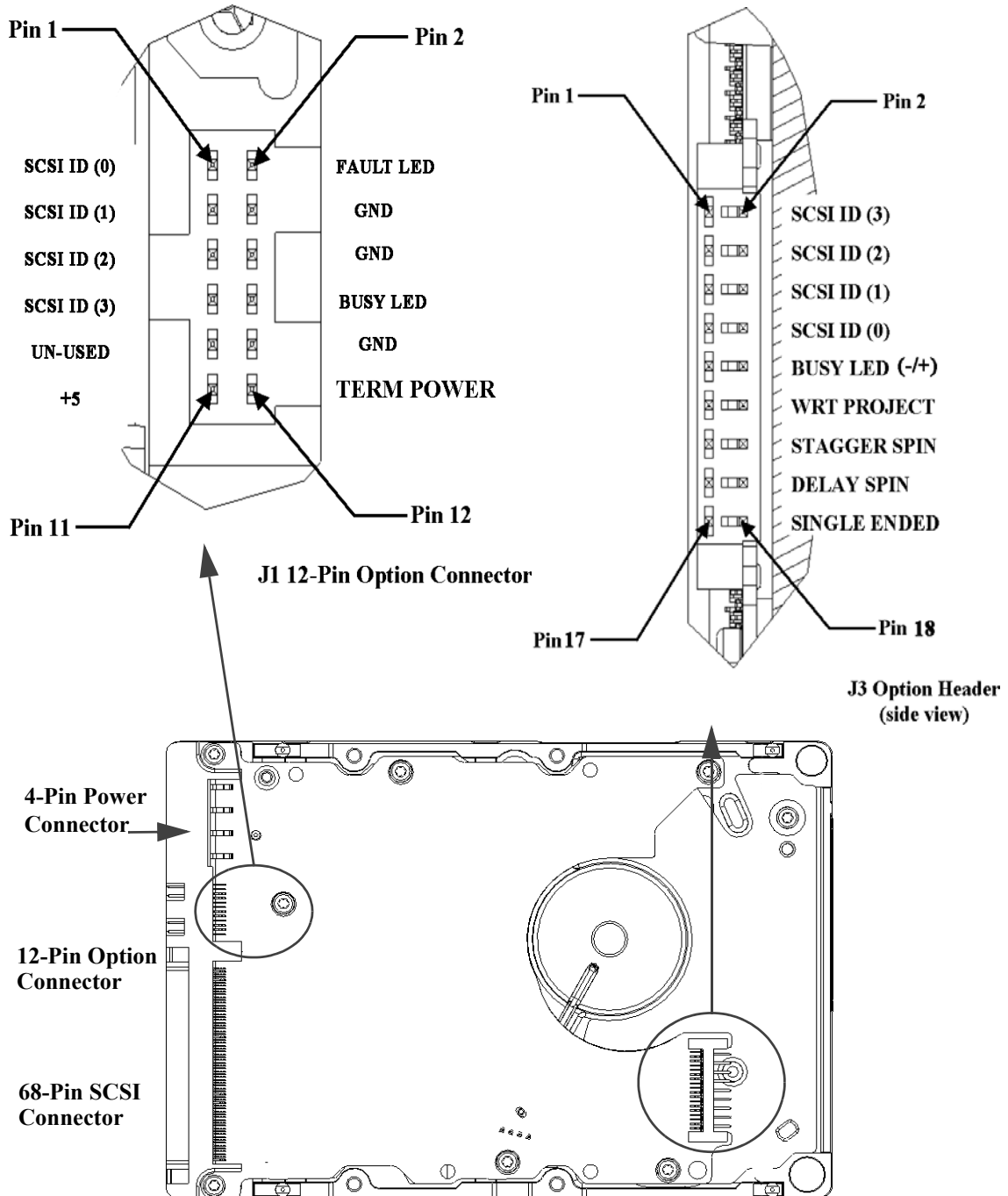
Figure 3-3 Jumper Locations on the 68-Pin Wide SCSI Drive PCB
