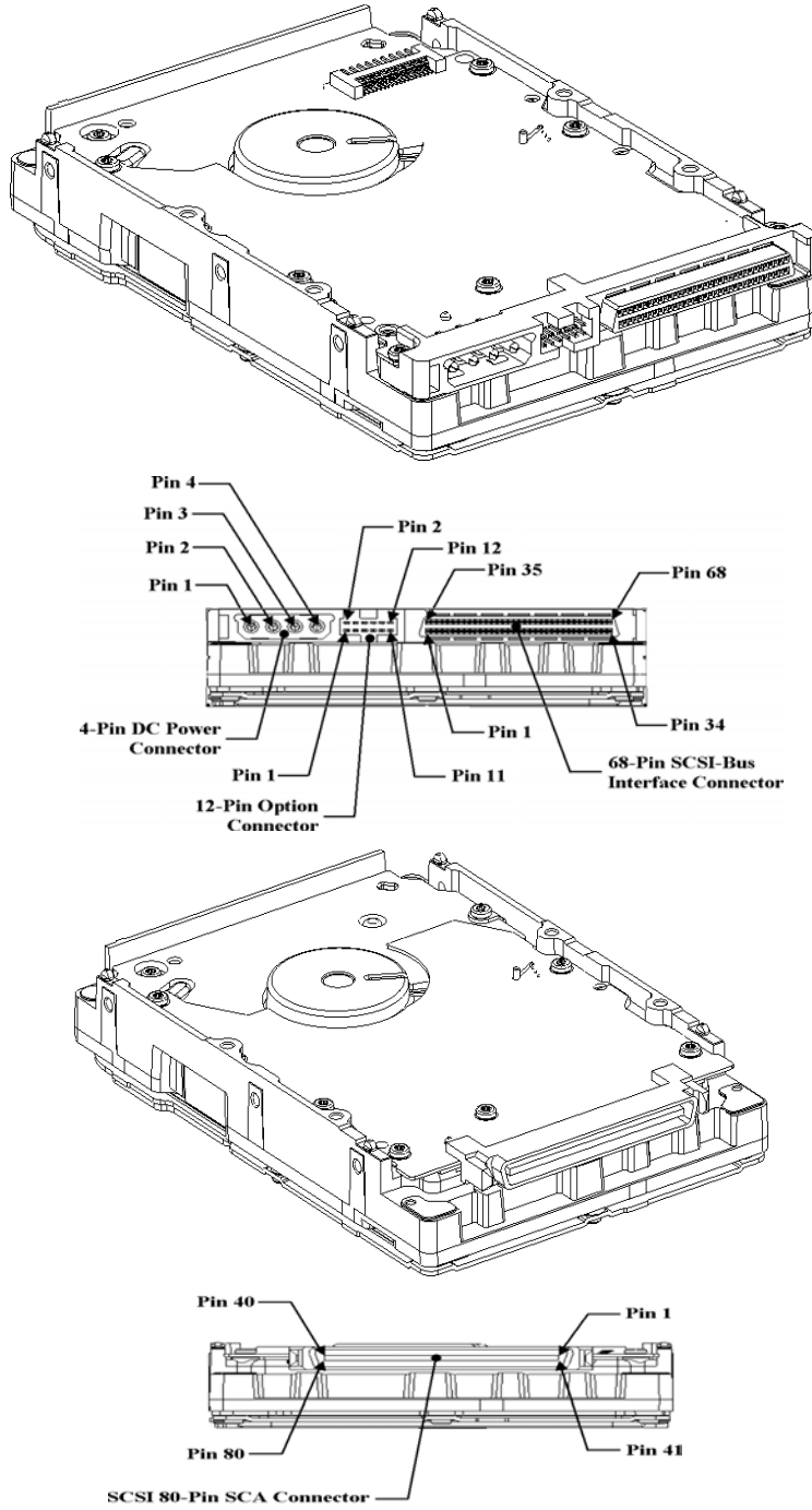
Figure 3-5 J1 Interface Connector Configurations
